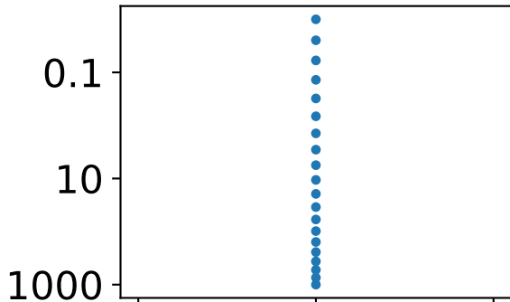
fixpoint=0.7, squeeze=0.5
