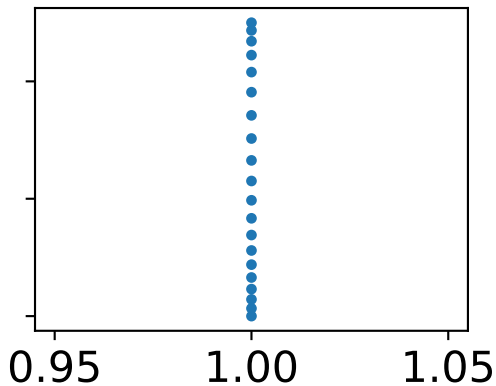
fixpoint=0.7, squeeze=1.5
