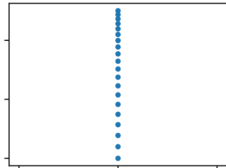
fixpoint=0.7, squeeze=1.5
