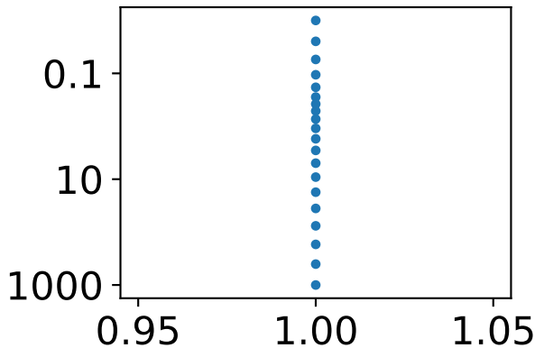
fixpoint=0.7, squeeze=0.5
